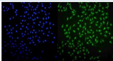
Immunofluorescent staining of FFPE human U-2 OS cells with UHRF1 antibody (green) and DAPI nuclear stain (blue). HIER: steam section in pH6 citrate buffer for 20 min.
