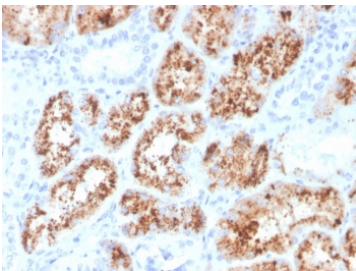
IHC staining of FFPE human kidney with RBP4 antibody. HIER: boil tissue sections in pH 9 10mM Tris with 1mM EDTA for 20 min and allow to cool before testing.
